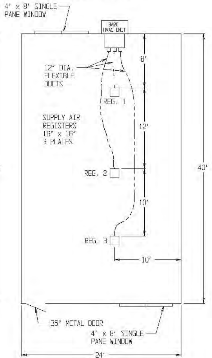
FIGURE 2 DUCT SYSTEM
